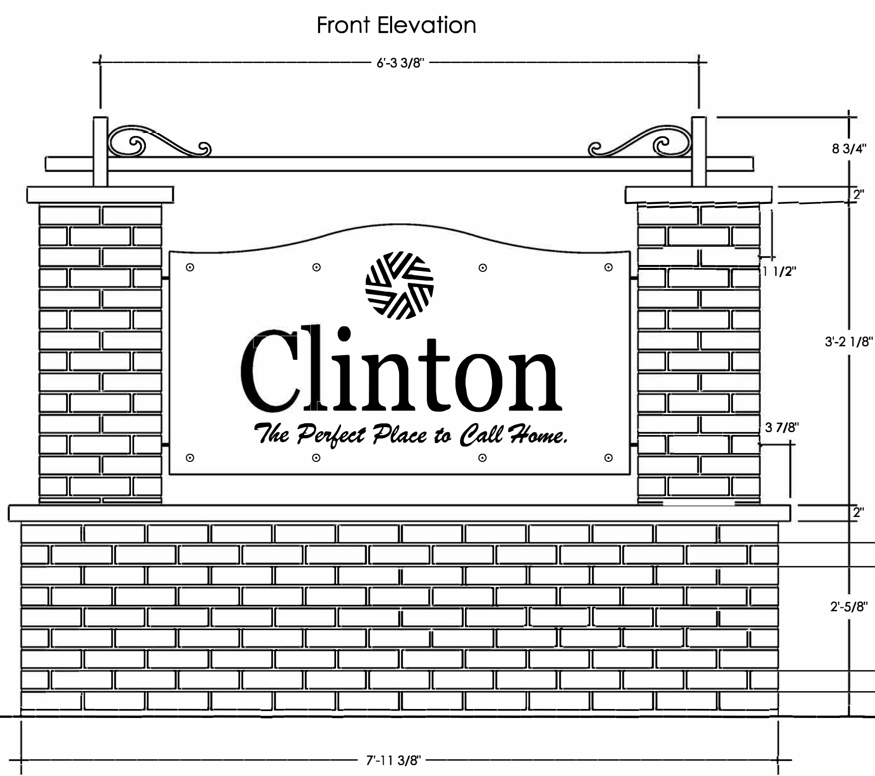
1 Clinton Gateway Sign Details 1" = 1'-0"
